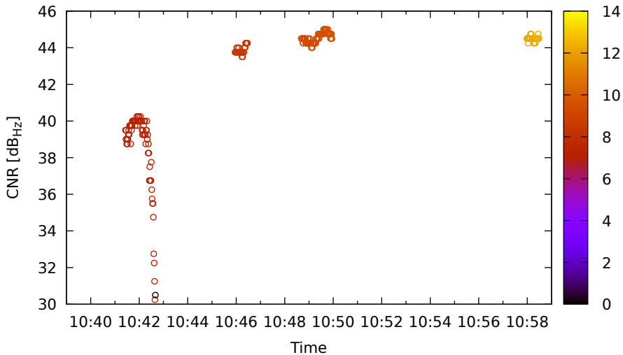
Timeline for E36 (E5b) on LeicaGS18 - DOY 263
