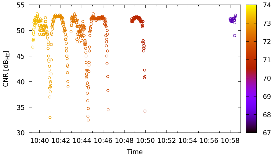
Timeline for G03 (L1) on LeicaGS18 - DOY 263
