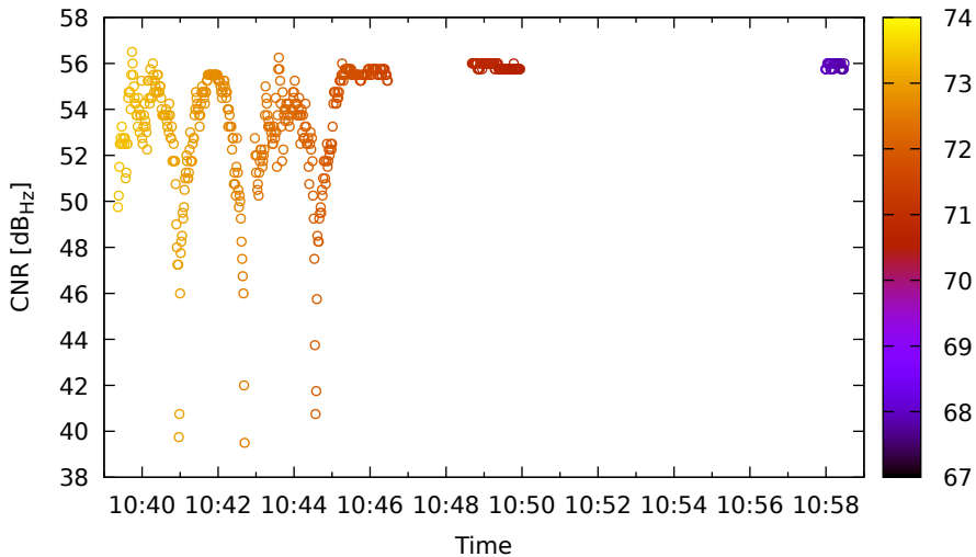
Timeline for G03 (L5) on LeicaGS18 - DOY 263
