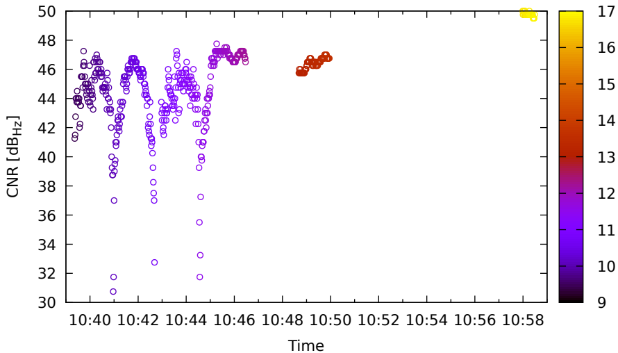
Timeline for G06 (L5) on LeicaGS18 - DOY 263
