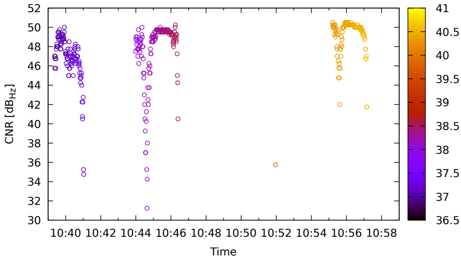
Timeline for C28 (B1) on LeicaGS18 - DOY 263
