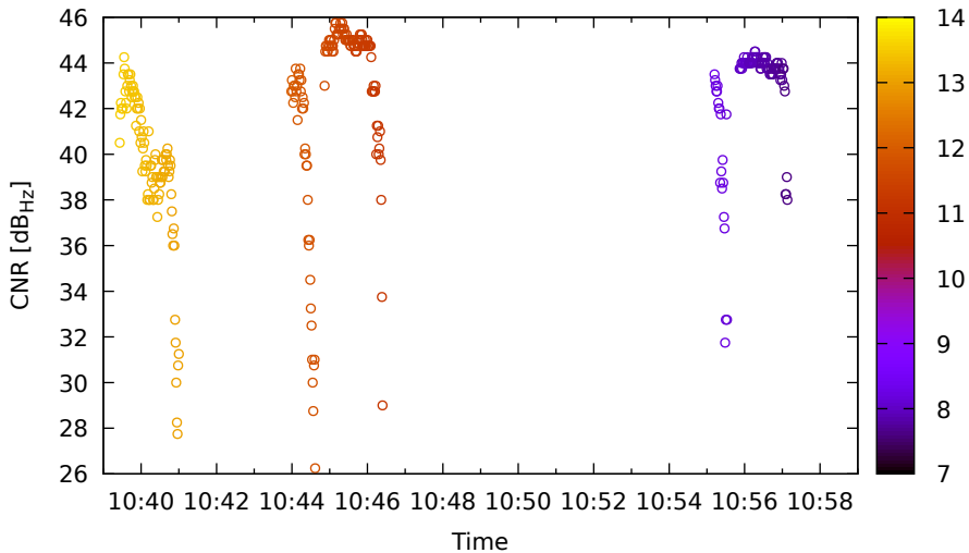
Timeline for E33 (E1) on LeicaGS18 - DOY 263
