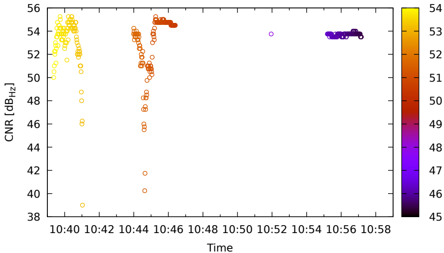
Timeline for G01 (L5) on LeicaGS18 - DOY 263
