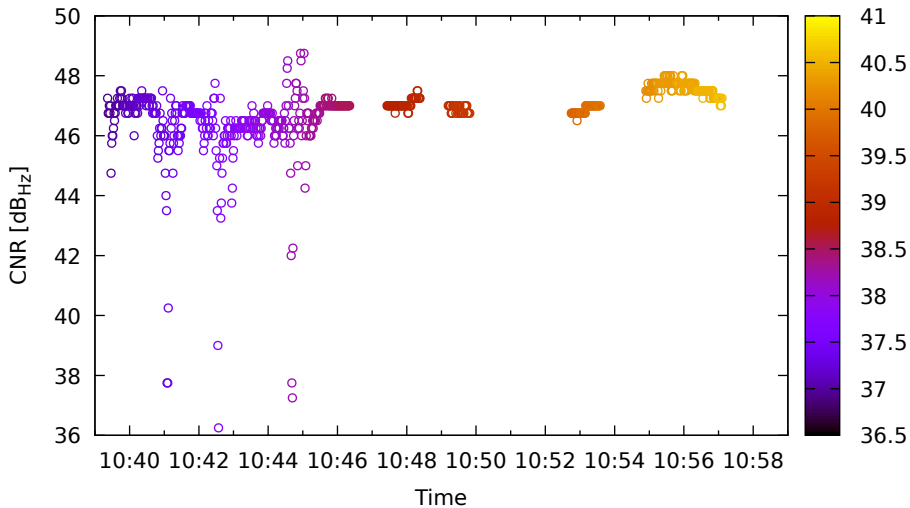
Timeline for C28 (B3) on LeicaGS18 - DOY 263
