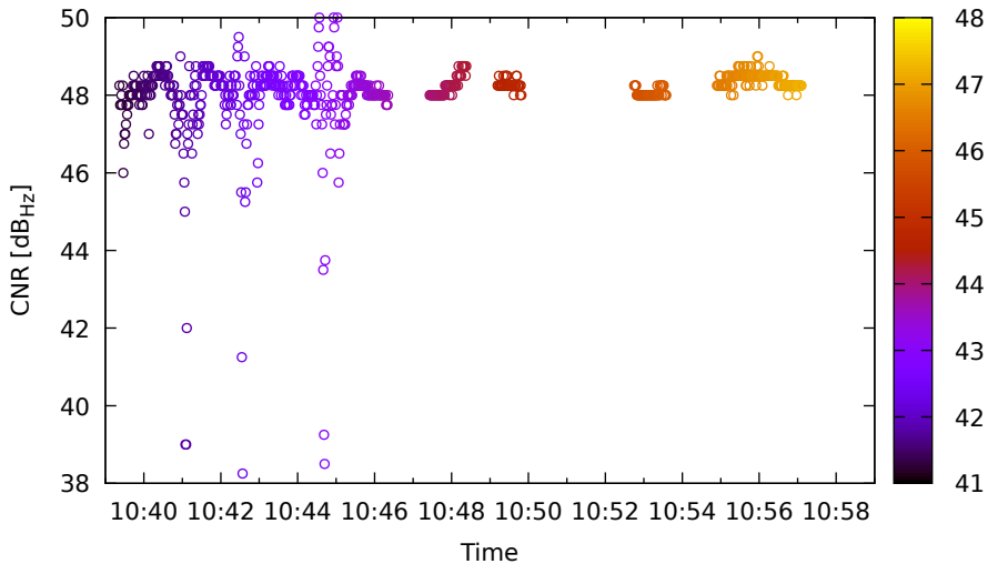
Timeline for C33 (B3) on LeicaGS18 - DOY 263
