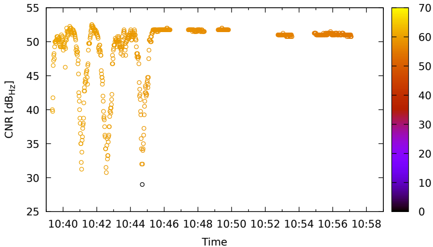
Timeline for E19 (E5) on LeicaGS18 - DOY 263
