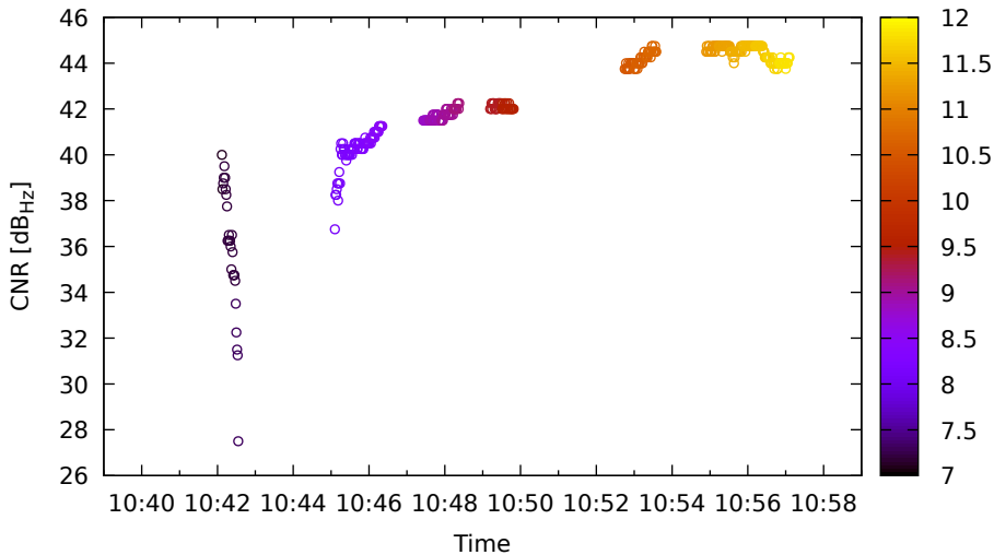
Timeline for E36 (E5a) on LeicaGS18 - DOY 263
