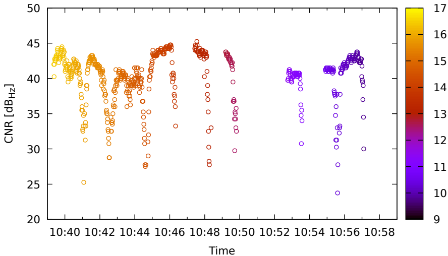
Timeline for G22 (L1) on LeicaGS18 - DOY 263
