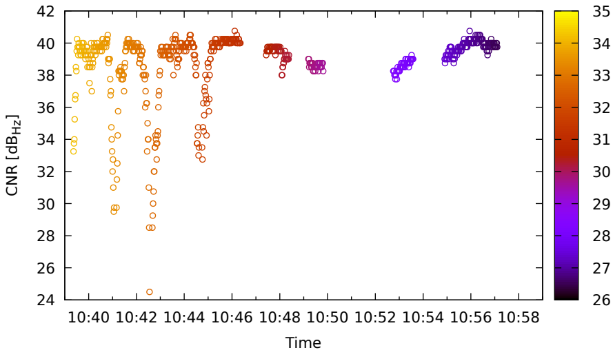
Timeline for R01 (G2) on LeicaGS18 - DOY 263
