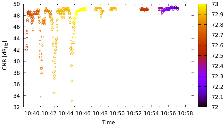
Timeline for R02 (G2) on LeicaGS18 - DOY 263
