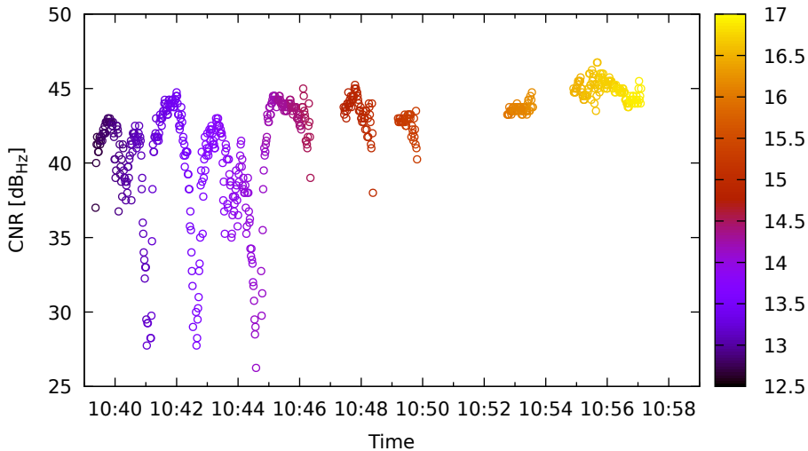
Timeline for R11 (G1) on LeicaGS18 - DOY 263
