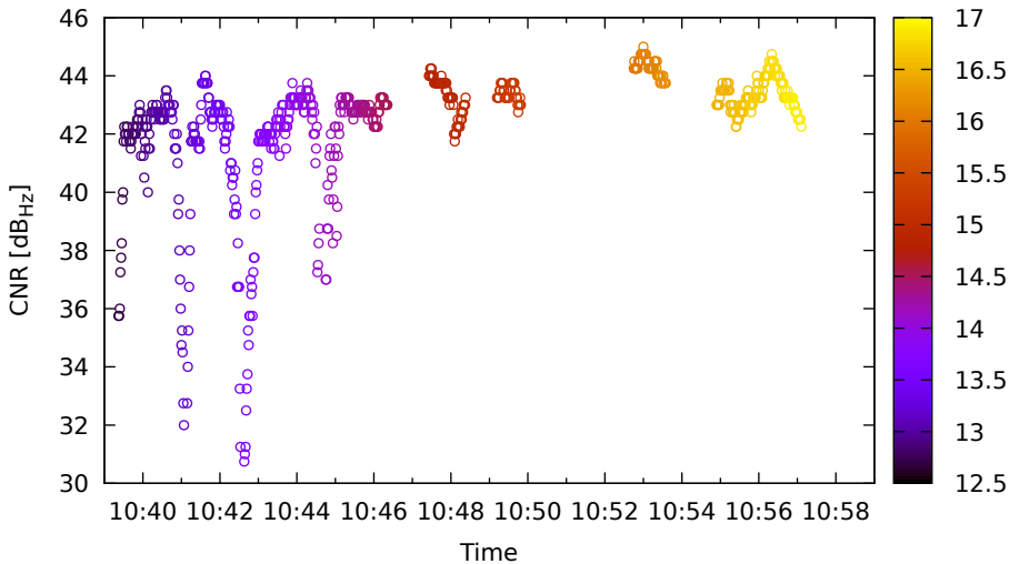
Timeline for R11 (G2) on LeicaGS18 - DOY 263
