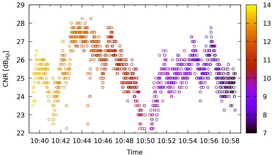
Timeline for E33 (E5a) on SamsungS20 - DOY 263
