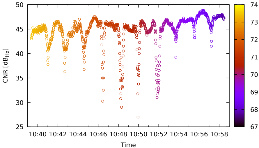
Timeline for G03 (L1) on SamsungS20 - DOY 263
