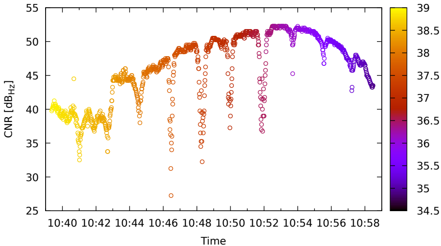
Timeline for G17 (L1) on SamsungS20 - DOY 263
