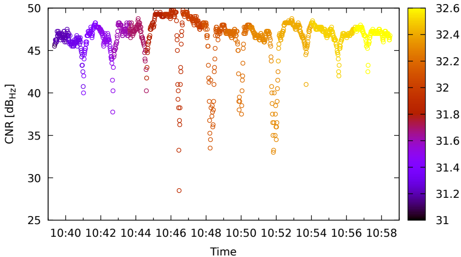
Timeline for G19 (L1) on SamsungS20 - DOY 263
