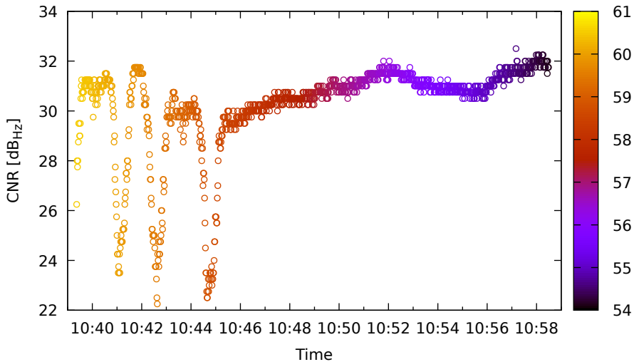
Timeline for E19 (E5a) on Xiaomi11T - DOY 263
