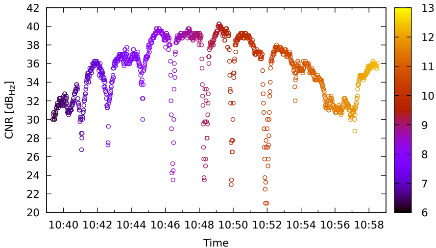
Timeline for E36 (E1) on Xiaomi11T - DOY 263
