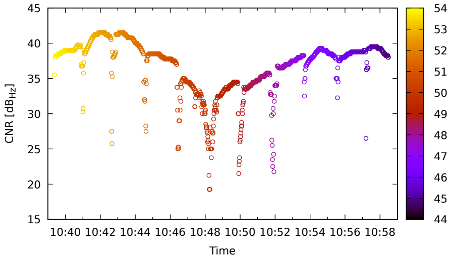
Timeline for G01 (L1) on Xiaomi11T - DOY 263
