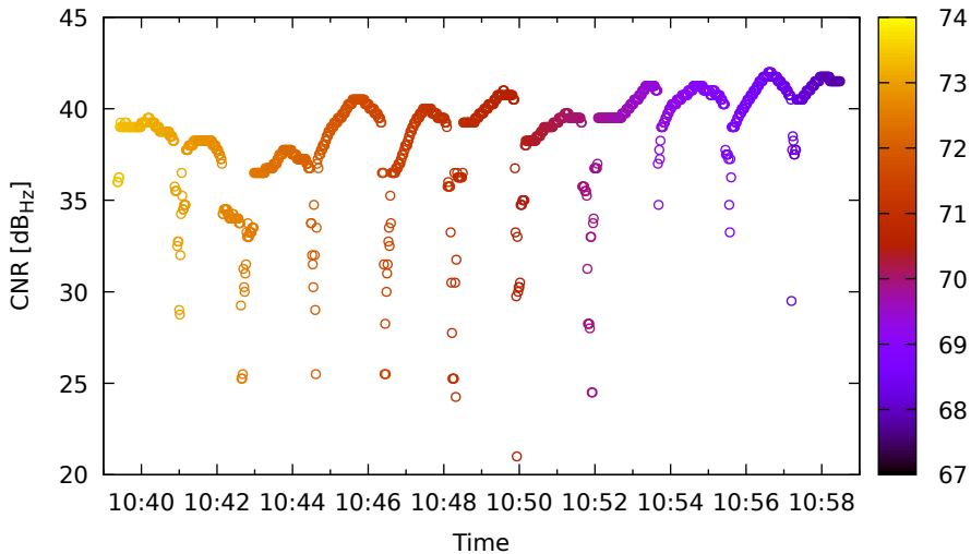
Timeline for G03 (L1) on Xiaomi11T - DOY 263
