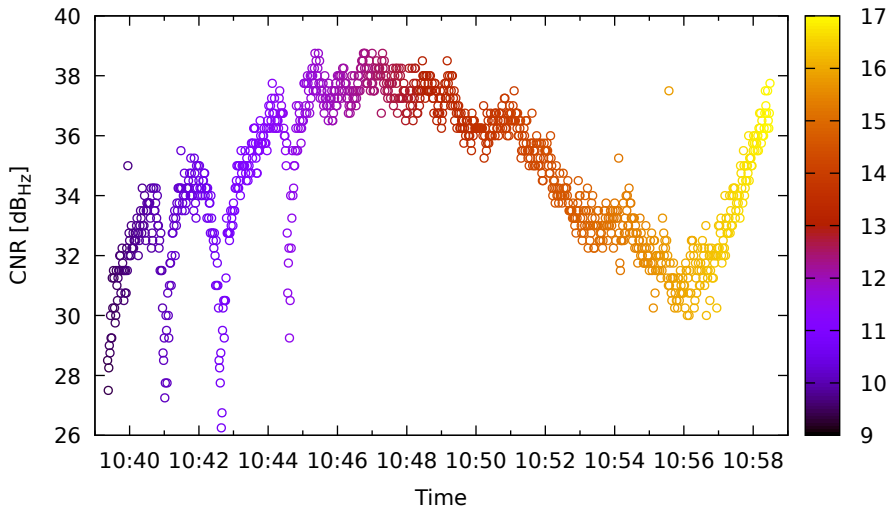
Timeline for G06 (L5) on Xiaomi11T - DOY 263
