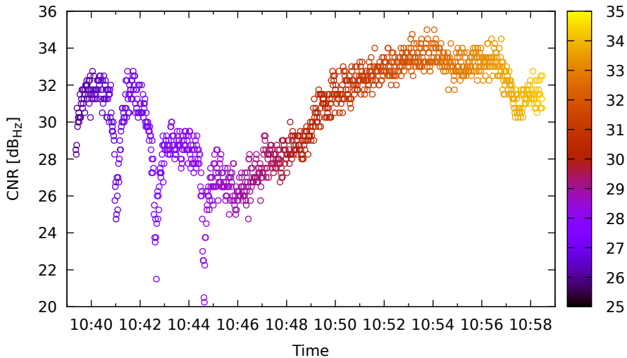
Timeline for G09 (L5) on Xiaomi11T - DOY 263
