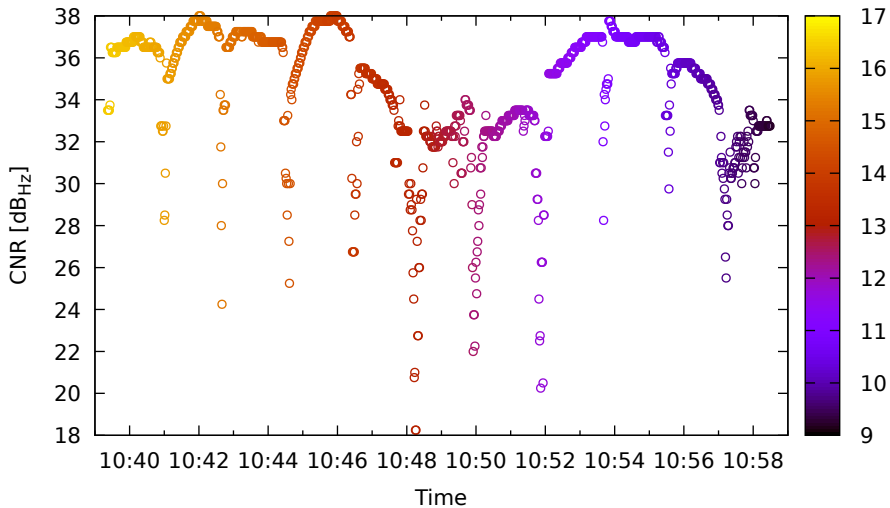
Timeline for G22 (L1) on Xiaomi11T - DOY 263
