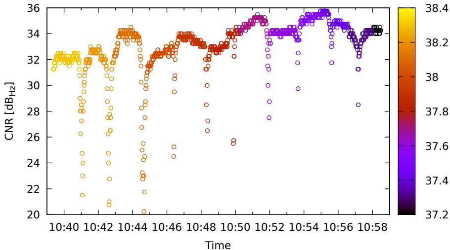
Timeline for C09 (B1) on XiaomiMi8 - DOY 263
