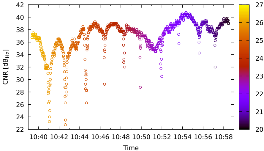
Timeline for C21 (B1) on XiaomiMi8 - DOY 263
