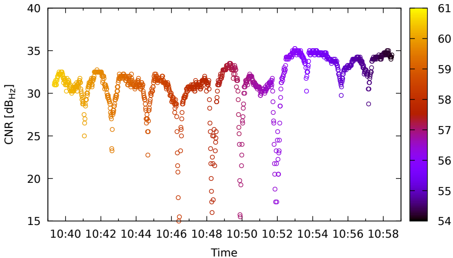
Timeline for E19 (E1) on XiaomiMi8 - DOY 263
