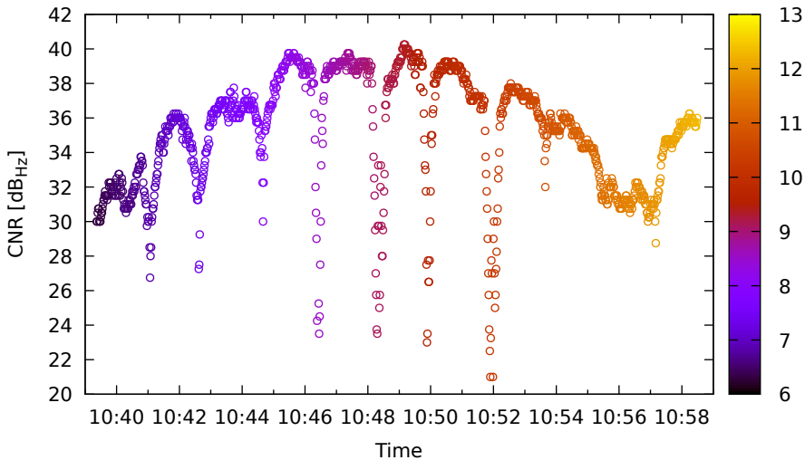
Timeline for E36 (E1) on XiaomiMi8 - DOY 263
