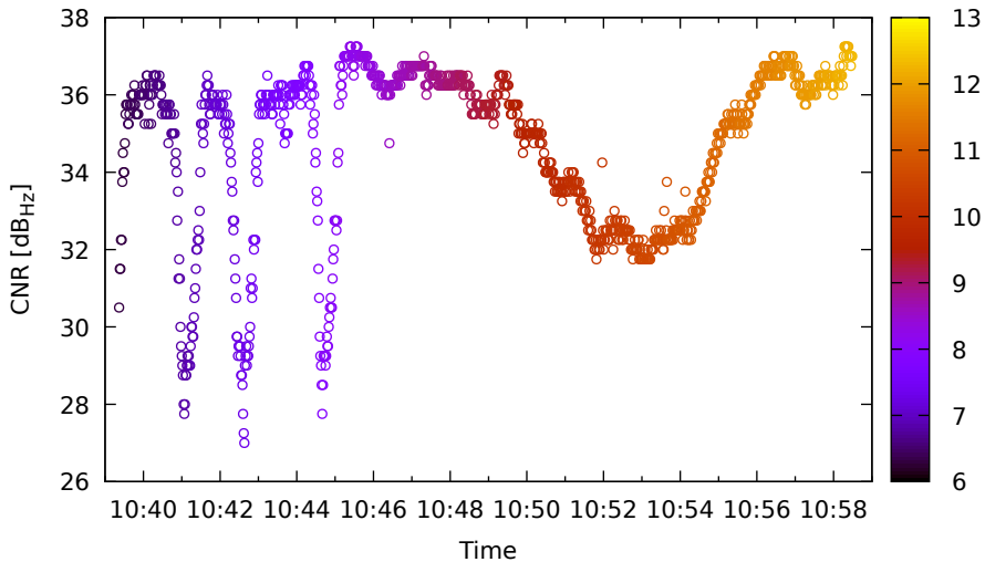
Timeline for E36 (E5a) on XiaomiMi8 - DOY 263
