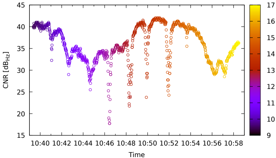
Timeline for G06 (L1) on XiaomiMi8 - DOY 263
