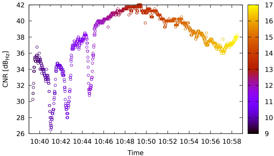
Timeline for G06 (L5) on XiaomiMi8 - DOY 263
