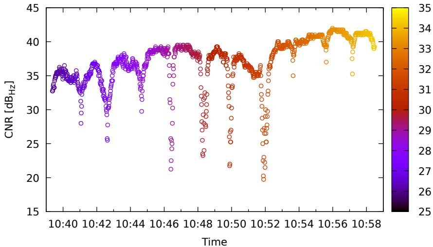
Timeline for G09 (L1) on XiaomiMi8 - DOY 263
