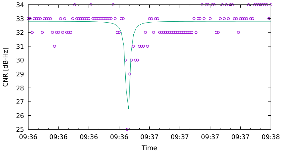
CNR fit for C06 on HuaweiP40 - drive 11 (DOY262)
