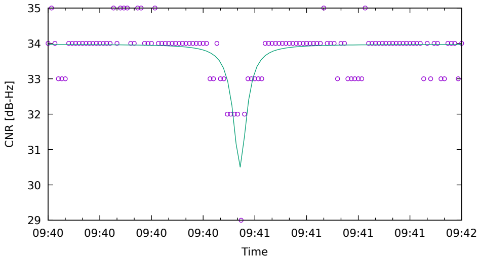
CNR fit for C06 on HuaweiP40 - drive 13 (DOY262)
