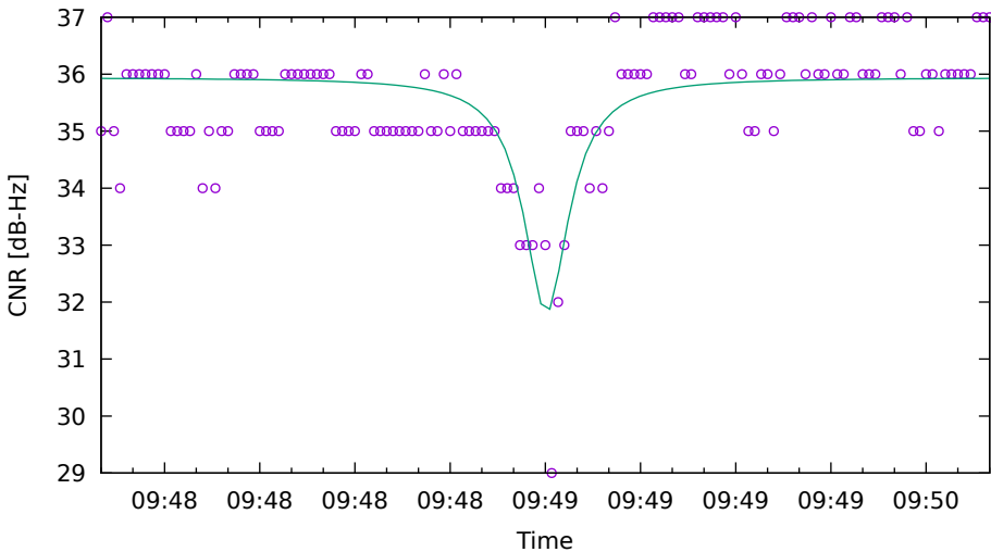
CNR fit for C06 on HuaweiP40 - drive 17 (DOY262)
