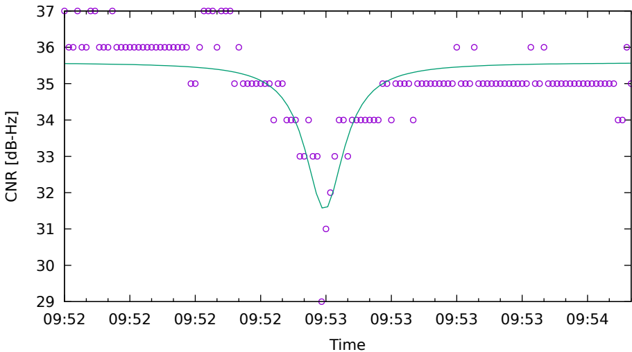
CNR fit for C06 on HuaweiP40 - drive 19 (DOY262)
