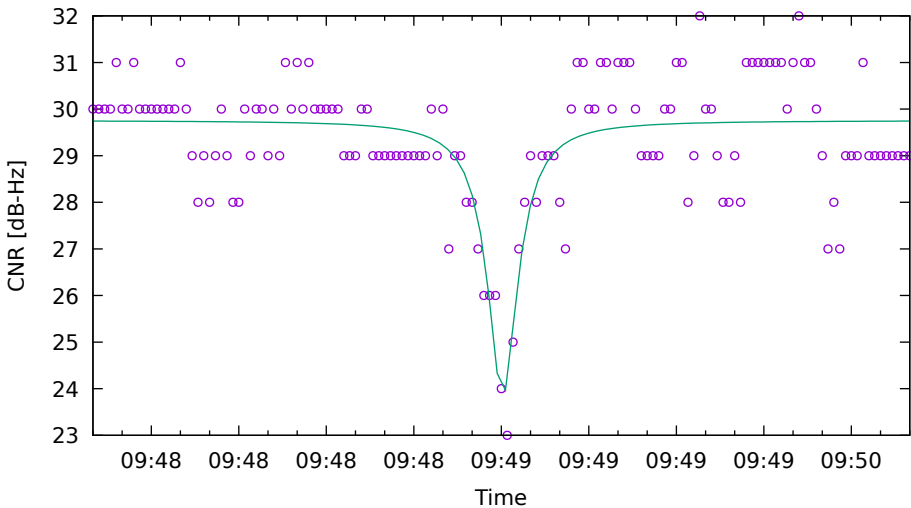
CNR fit for C09 on HuaweiP40 - drive 17 (DOY262)
