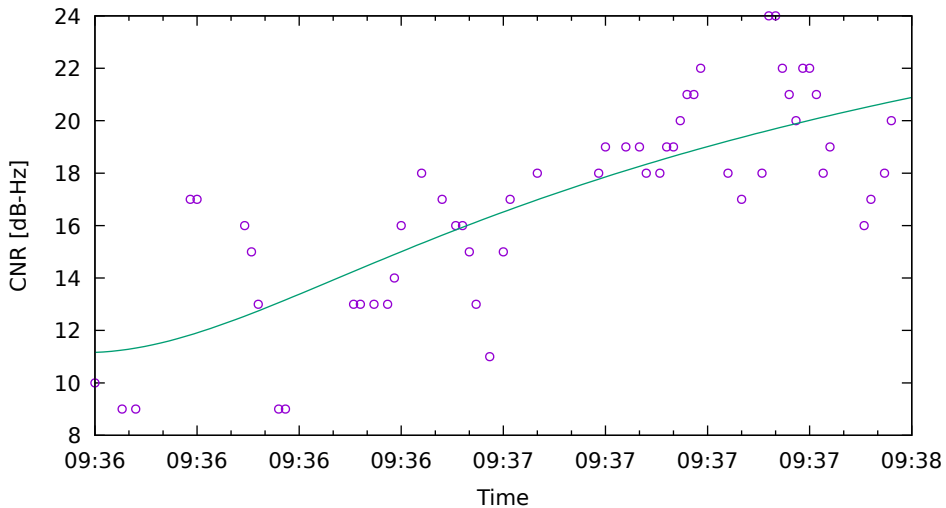
CNR fit for C11 on HuaweiP40 - drive 11 (DOY262)
