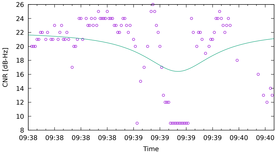
CNR fit for C11 on HuaweiP40 - drive 12 (DOY262)
