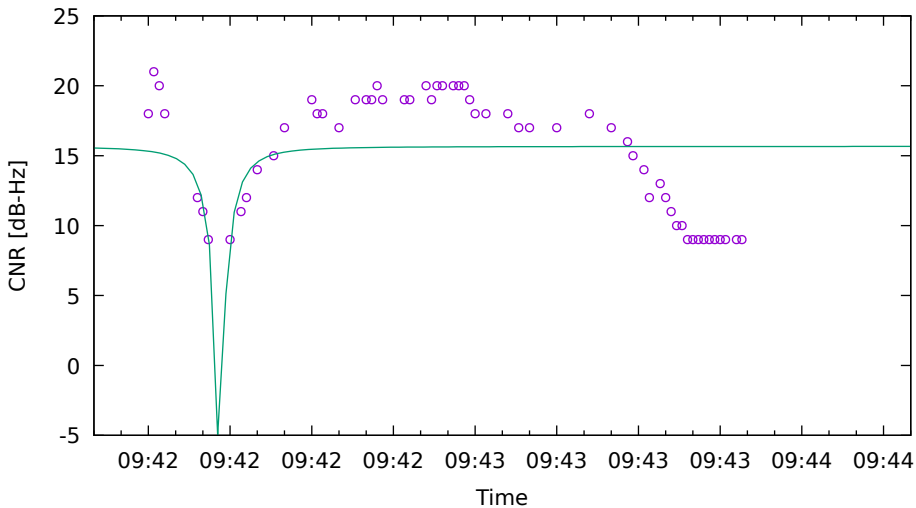
CNR fit for C11 on HuaweiP40 - drive 14 (DOY262)
