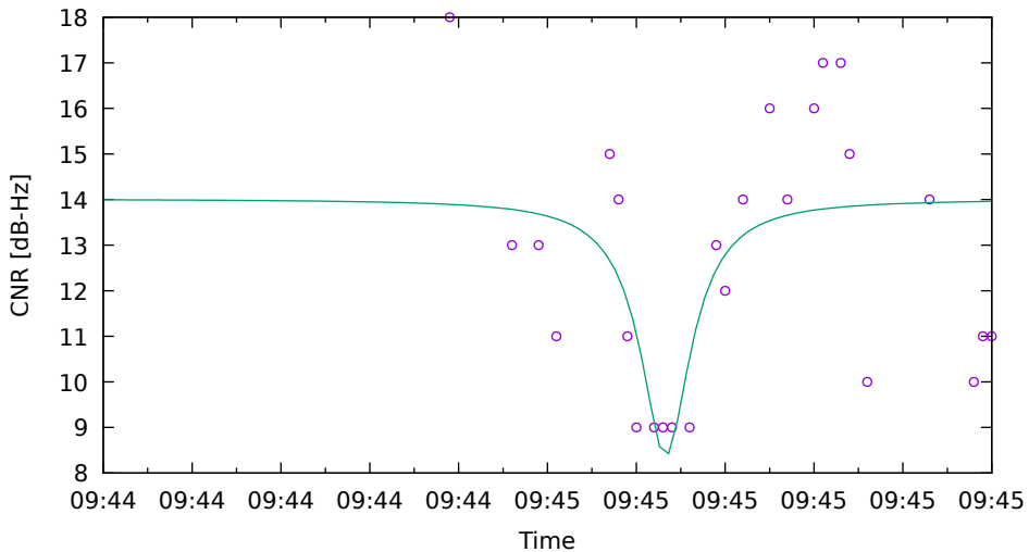
CNR fit for C11 on HuaweiP40 - drive 15 (DOY262)
