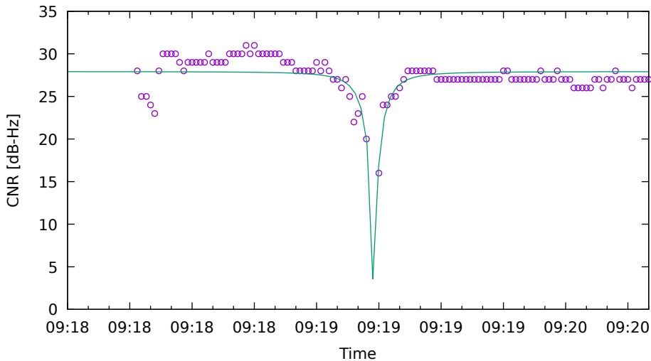
CNR fit for C11 on HuaweiP40 - drive 2 (DOY262)
