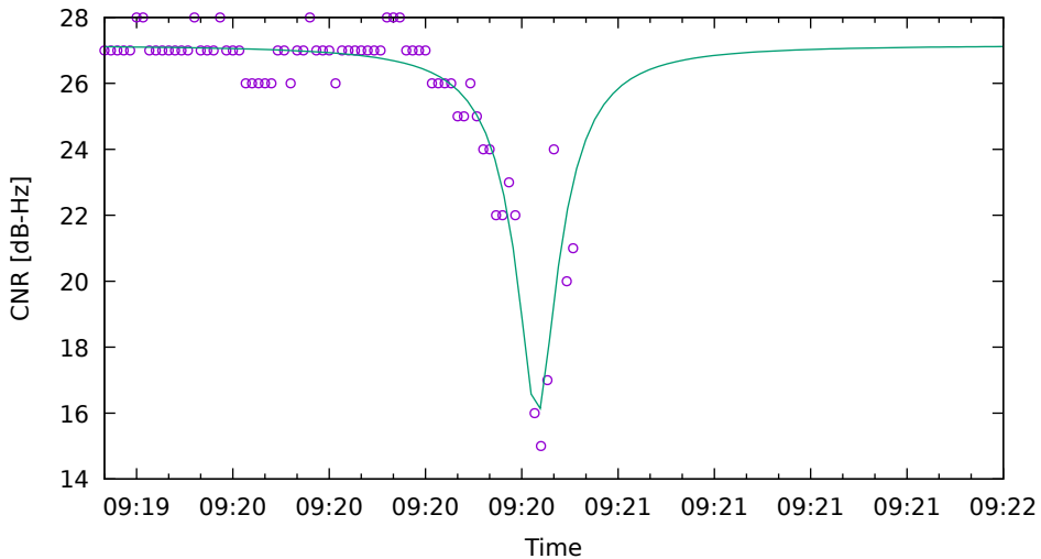
CNR fit for C11 on HuaweiP40 - drive 3 (DOY262)
