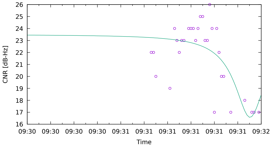
CNR fit for C11 on HuaweiP40 - drive 8 (DOY262)
