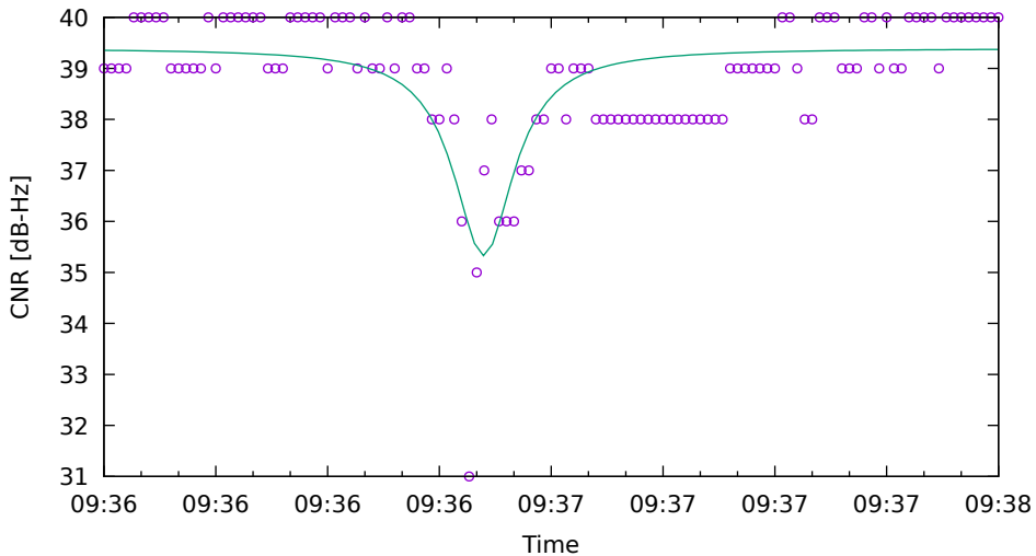
CNR fit for C16 on HuaweiP40 - drive 11 (DOY262)
