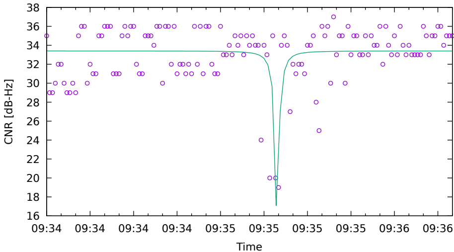
CNR fit for C27 on HuaweiP40 - drive 10 (DOY262)
