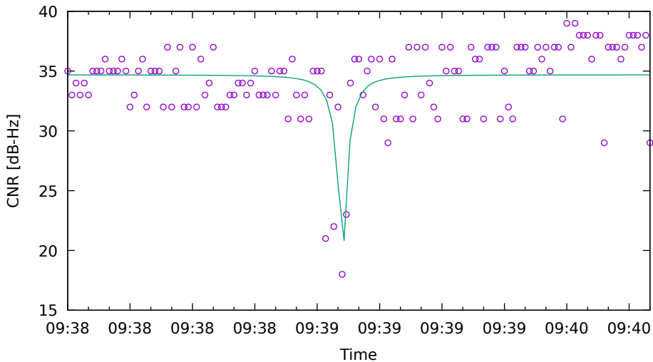
CNR fit for C27 on HuaweiP40 - drive 12 (DOY262)
